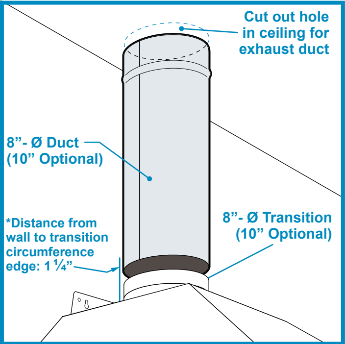
(Fig 7) *For 8" - Ø Transition. Distance from wall to transition circumference edge for 10" - Ø Transition will be 1/8". Use 8" or 10" round steel pipe (follow building codes in your area) to connect the exhaust on the hood to the ductwork above. Use aluminum tape to make all joints secure and air tight.
