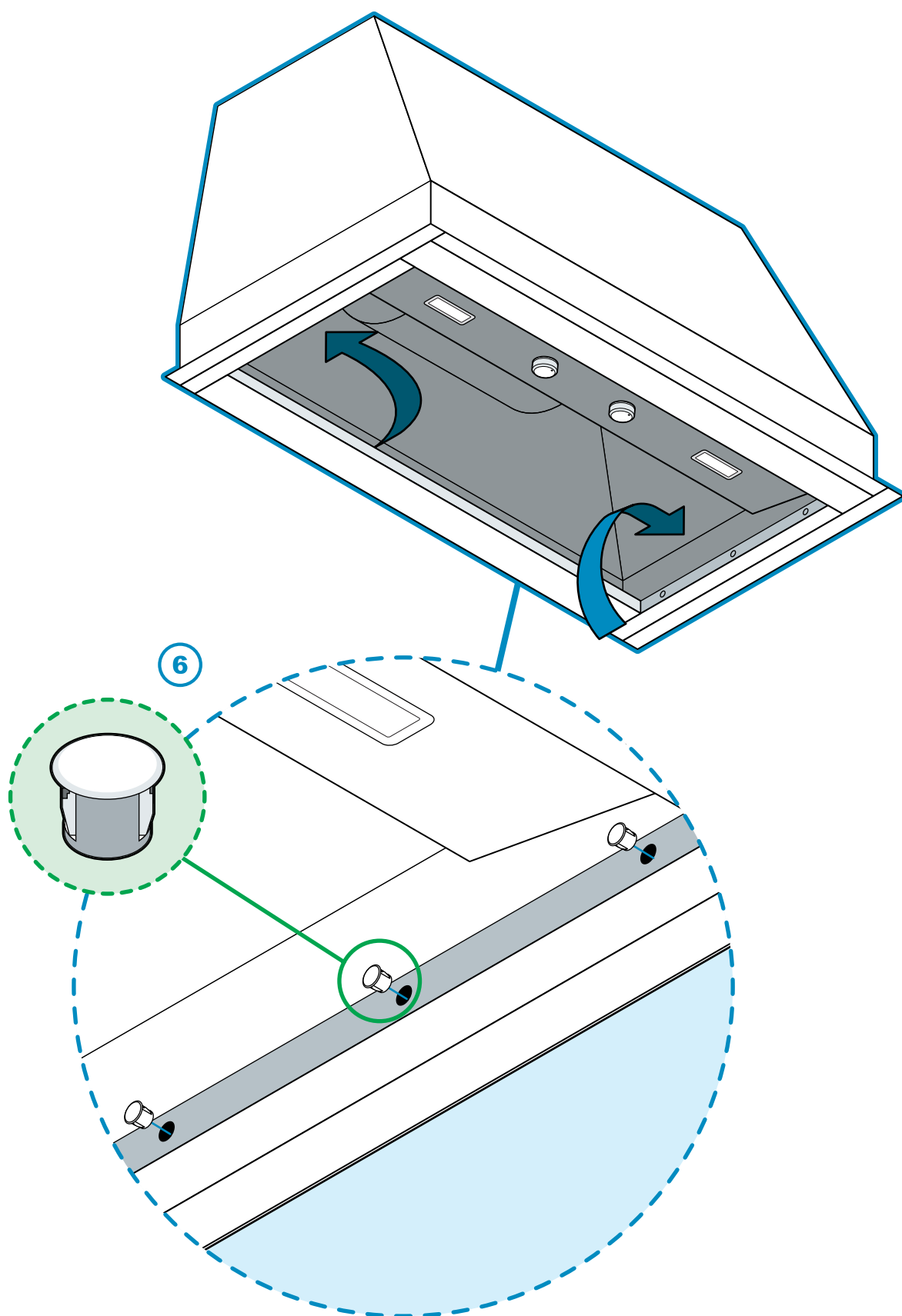
(Fig 6) After mounting range hood to side panels, insert caps into screw holes on both side walls inside the range hood.
