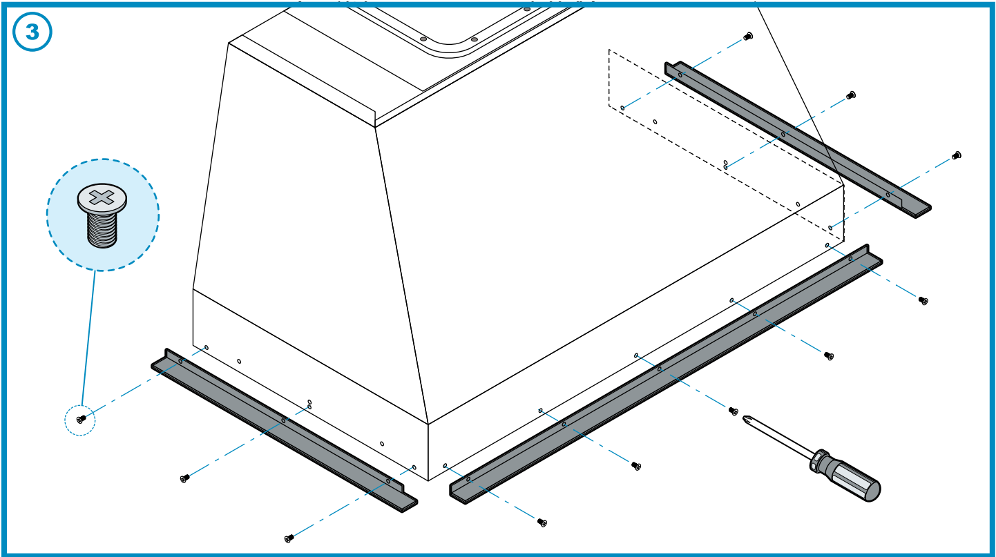
(Fig 3) Fasten trim pieces on to the front and sides of range hood using M4-4mm countersink screws. These trim pieces may not be necessary depending on the structure and material of housing or cabinet will be built in to.
