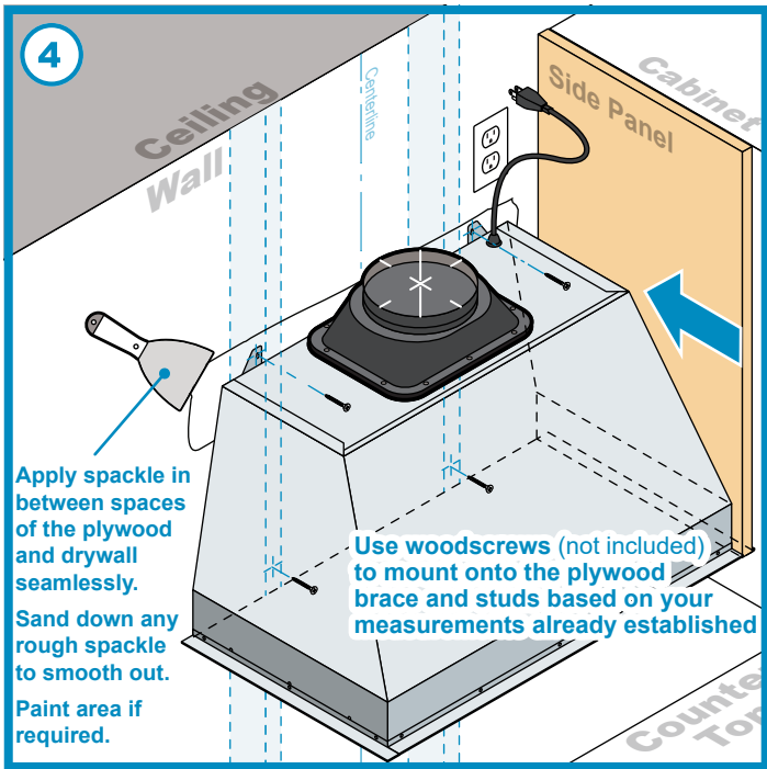
(Fig 4) Patch up the plywood brace area and sand down any rough areas. Use woodscrews (not included) to fasten range hood onto brace support and studs.
