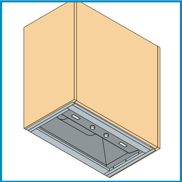
(Fig 8) Complete the build of the cabinet surround ensuring the lip of the range hood fits flush to the bottom of the cabinet.
