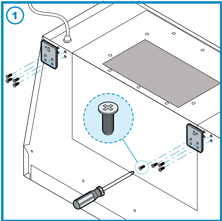
(Fig 1) Fasten installation plates using M5-5mm screws on to the back of the range hood.
