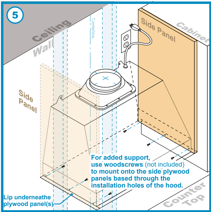
(Fig 5) Continue to fasten woodscrews (not included) to the side panels to secure the range hood. Ensure that the trim fits flush underneath the panels.
