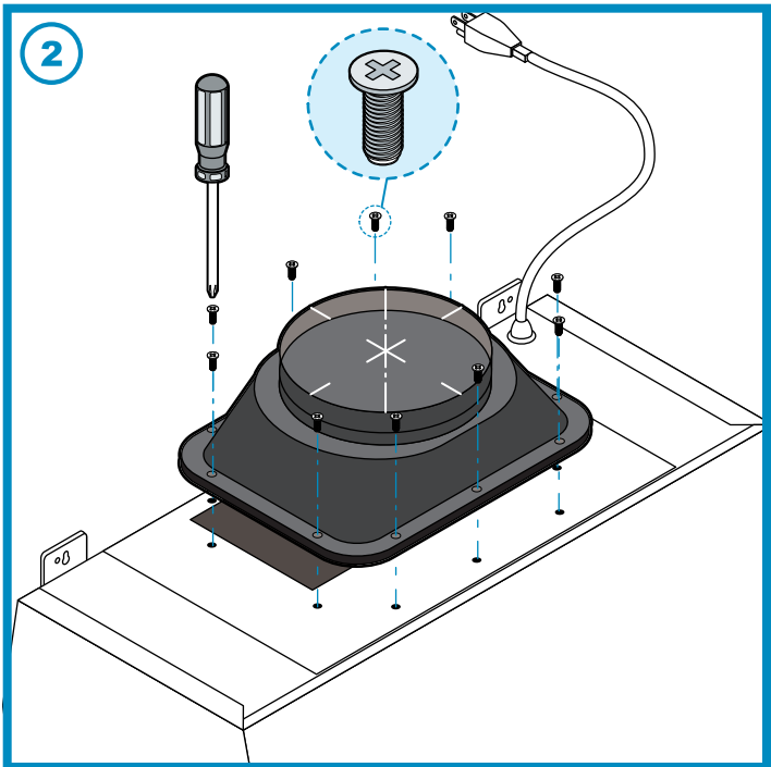
(Fig 2) Fasten on 8" - Ø Transition on to the top exhaust of range hood using M5-5mm screws (10" Optional).
