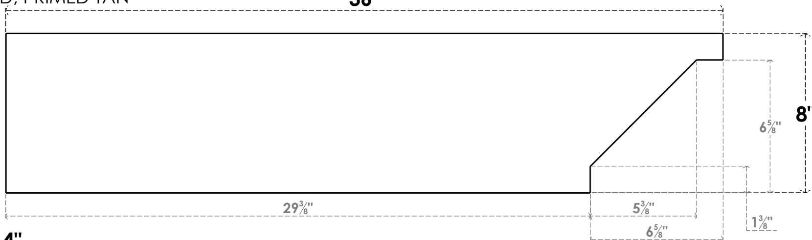
SIDE PROFILE
