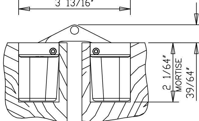
HINGE OPEN 180° TOP VIEW CUT AWAY
