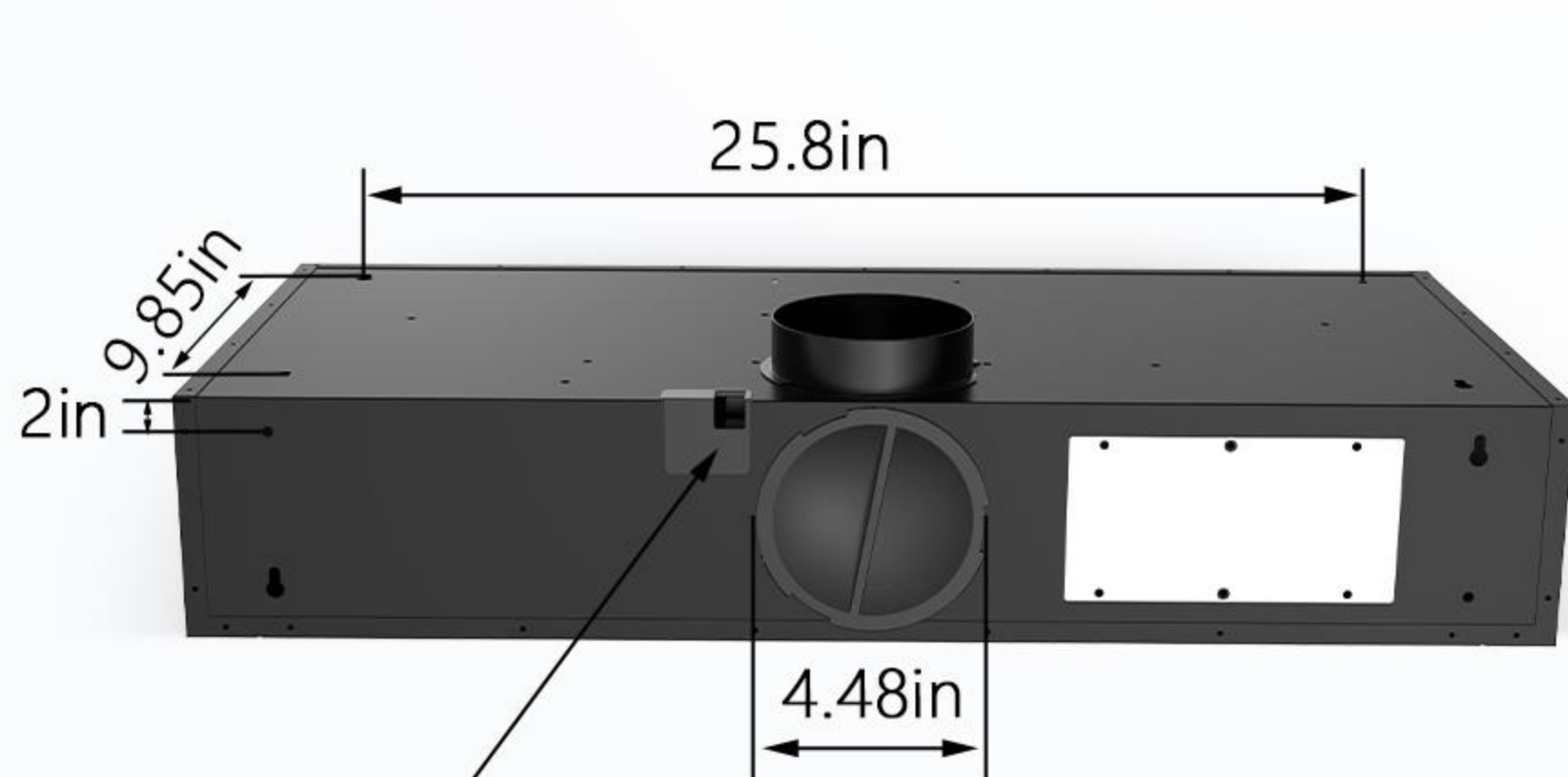
Location of 3-prong plug
