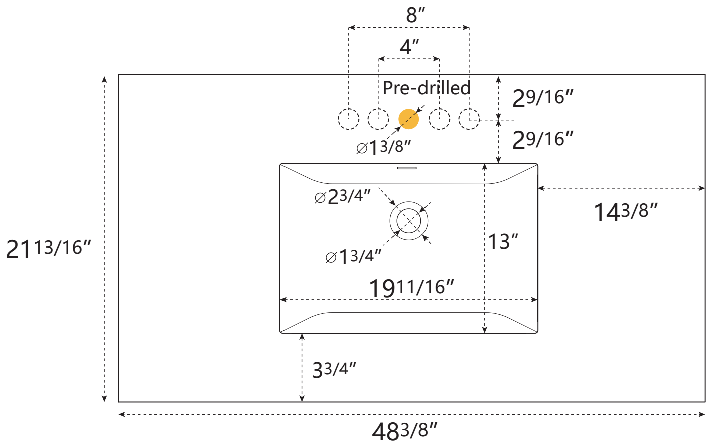
TOP VIEW
