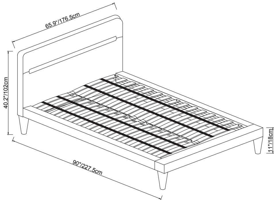
Product Dimension
