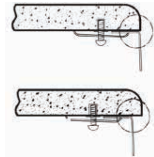
Flushed reveal - counter is flush with edge of sink (most popular)
