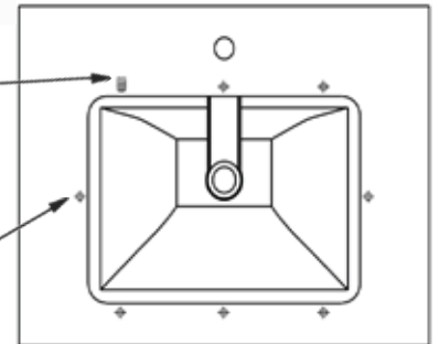
Evenly spaced drill holes, approx. 6" - 8" apart
