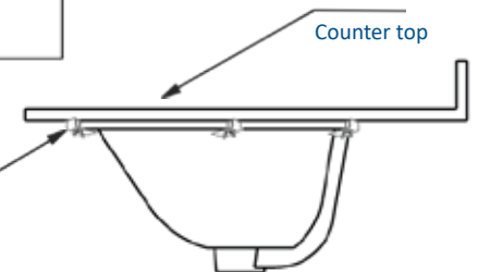
Loosely attached sink clips, and mounting brackets on to brass nut anchors using long bolt, washers and butterfly/wing nuts
