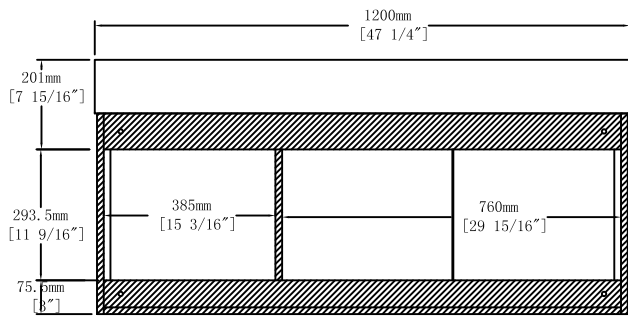
Back View
