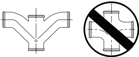
Recommended fitting type for back-to-back installations.
