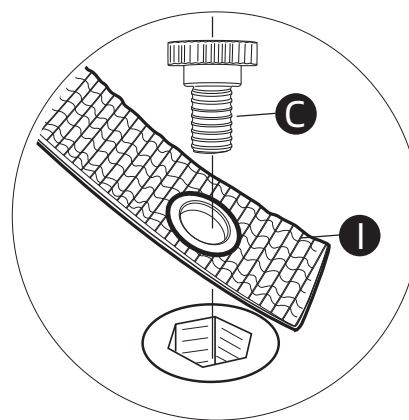
Anti-tipping device
