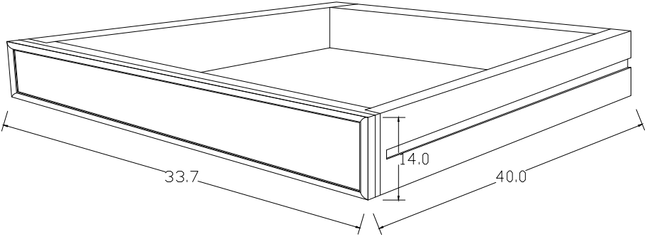
DRAWER DETAIL
