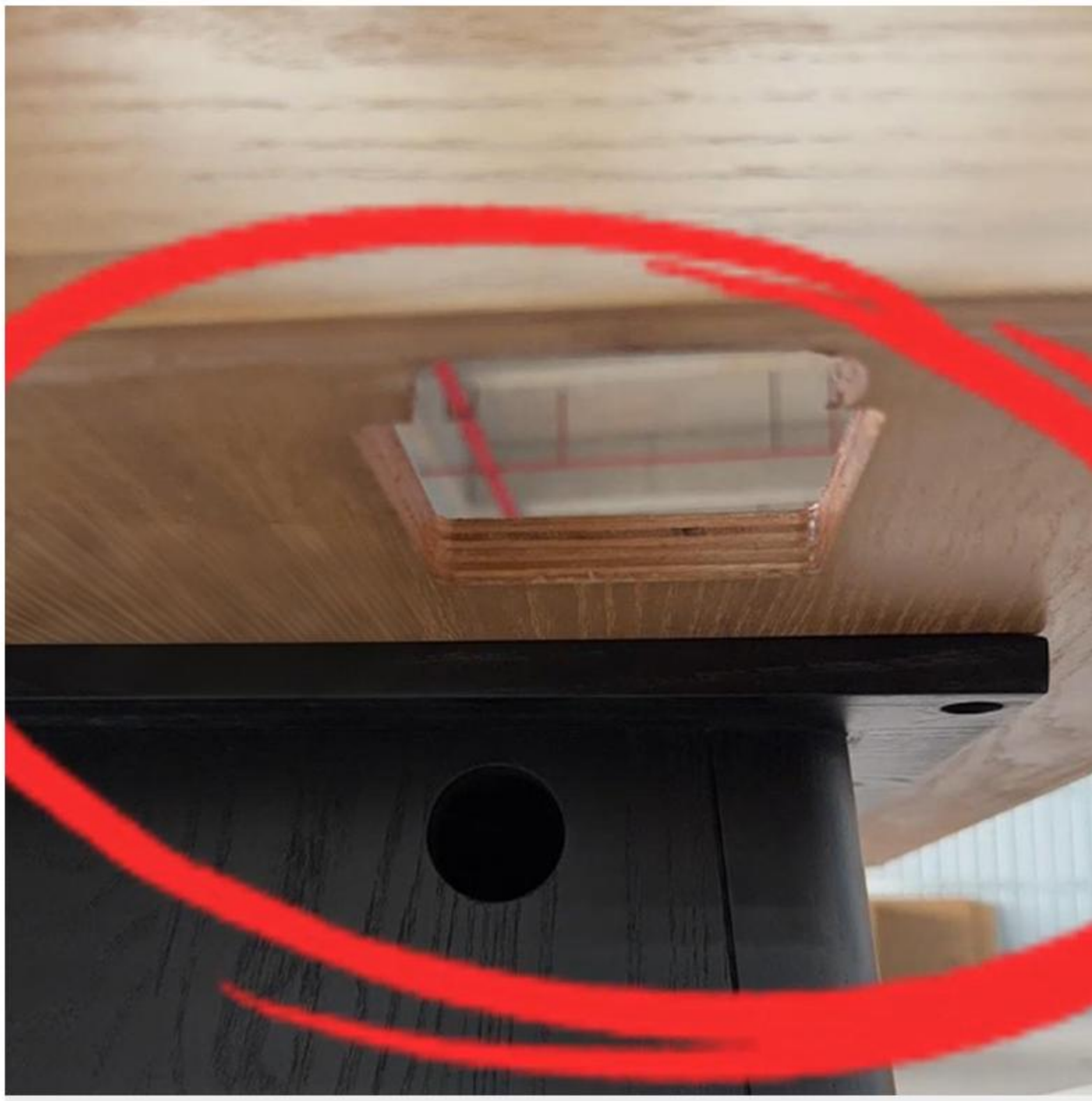
Note: The power cord hole on the table legs must face the same direction as the power cord hole on the frame.
