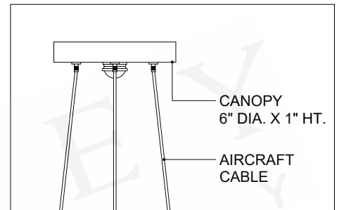
CANOPY DETAIL
