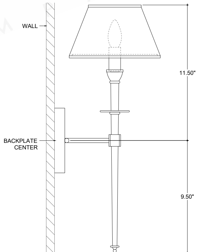
SIDE VIEW
