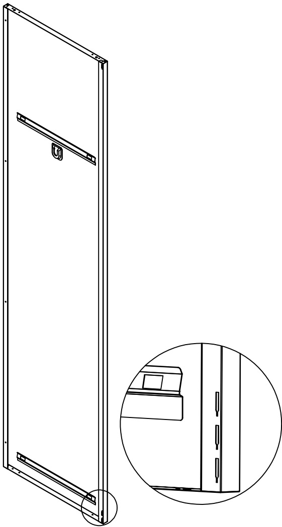
B:Right side panel
