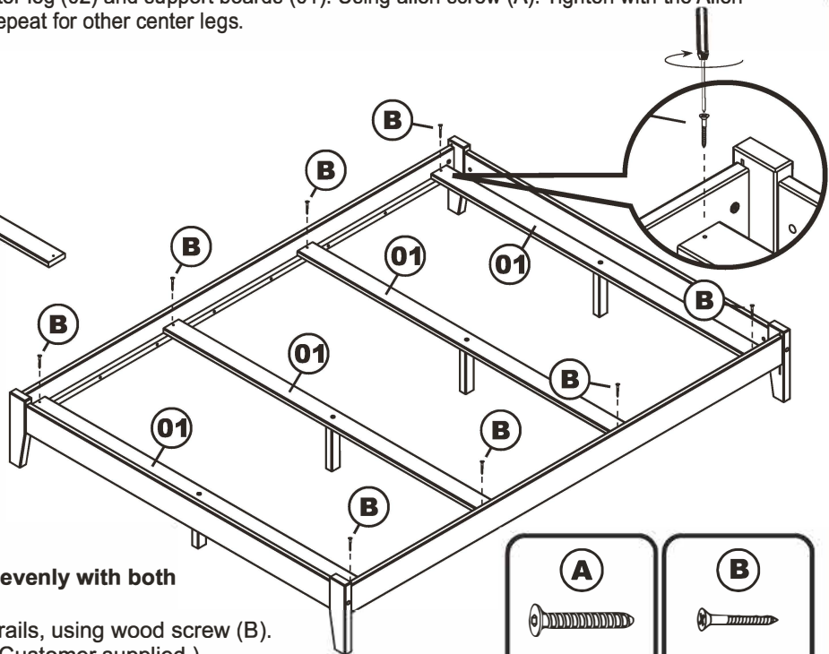
Allen screw
