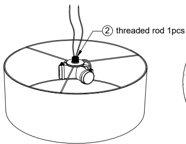
① light fixture 1pcs
