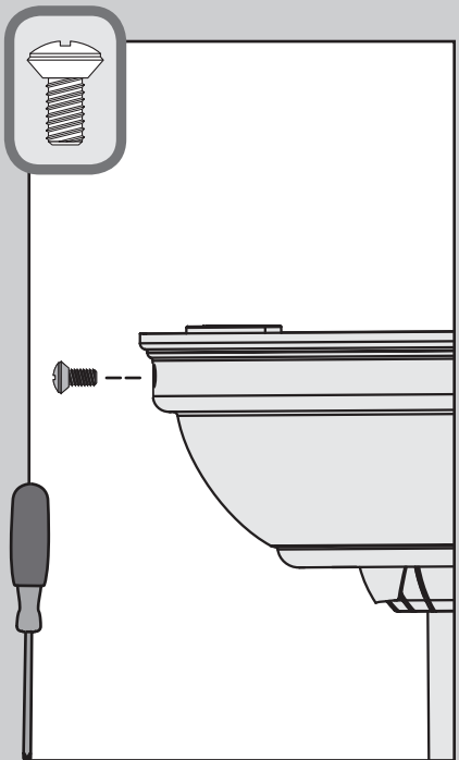
⊗ Install the two canopy screws found in the ● hardware bag.
