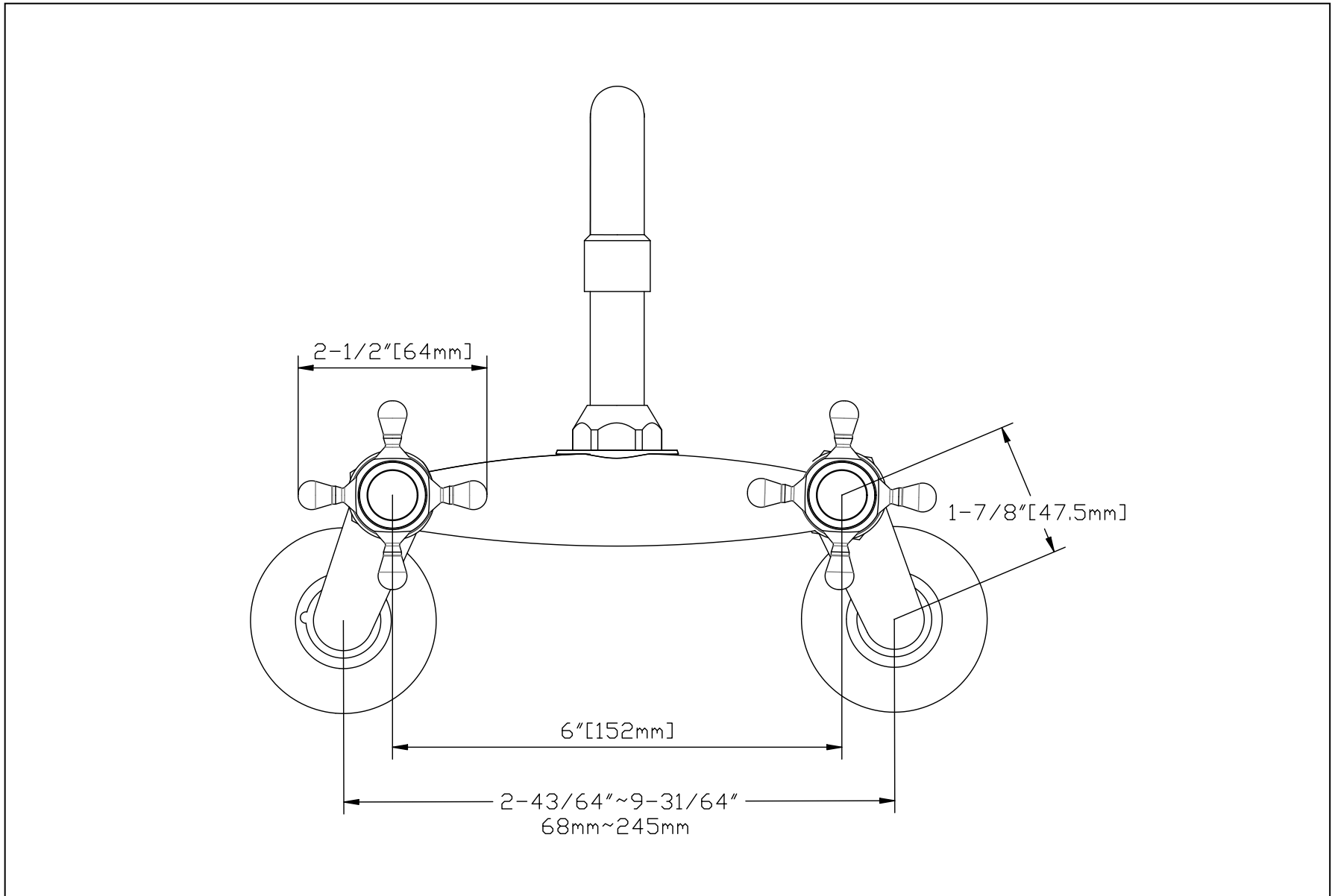
FRONT VIEW
