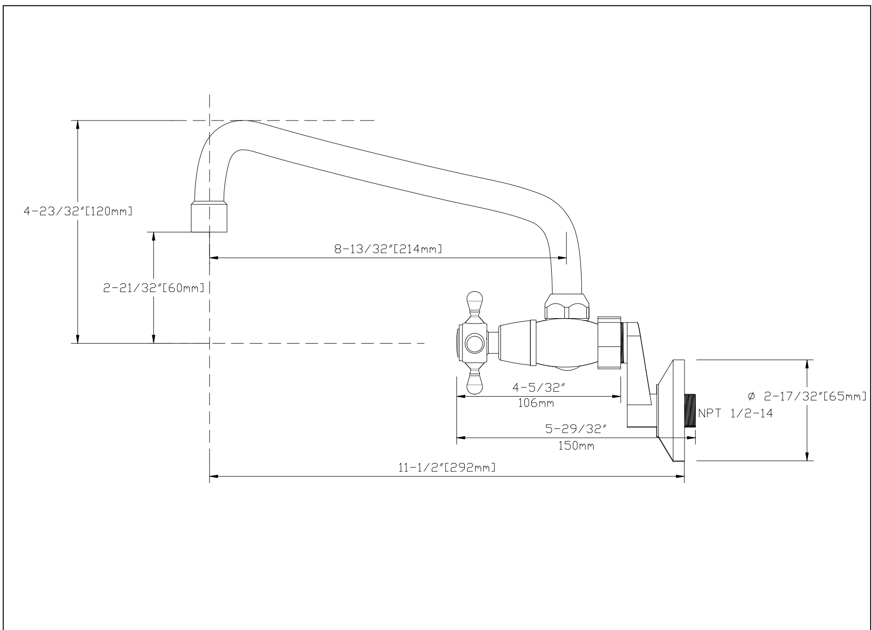
SIDE VIEW
