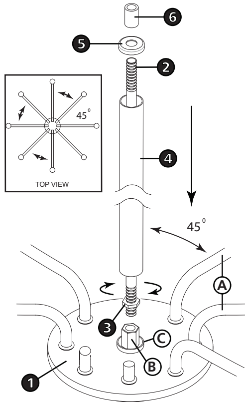
DRAWING 1 - ASSEMBLY
