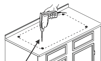
3/8" (10 mm) diameter drill bit
