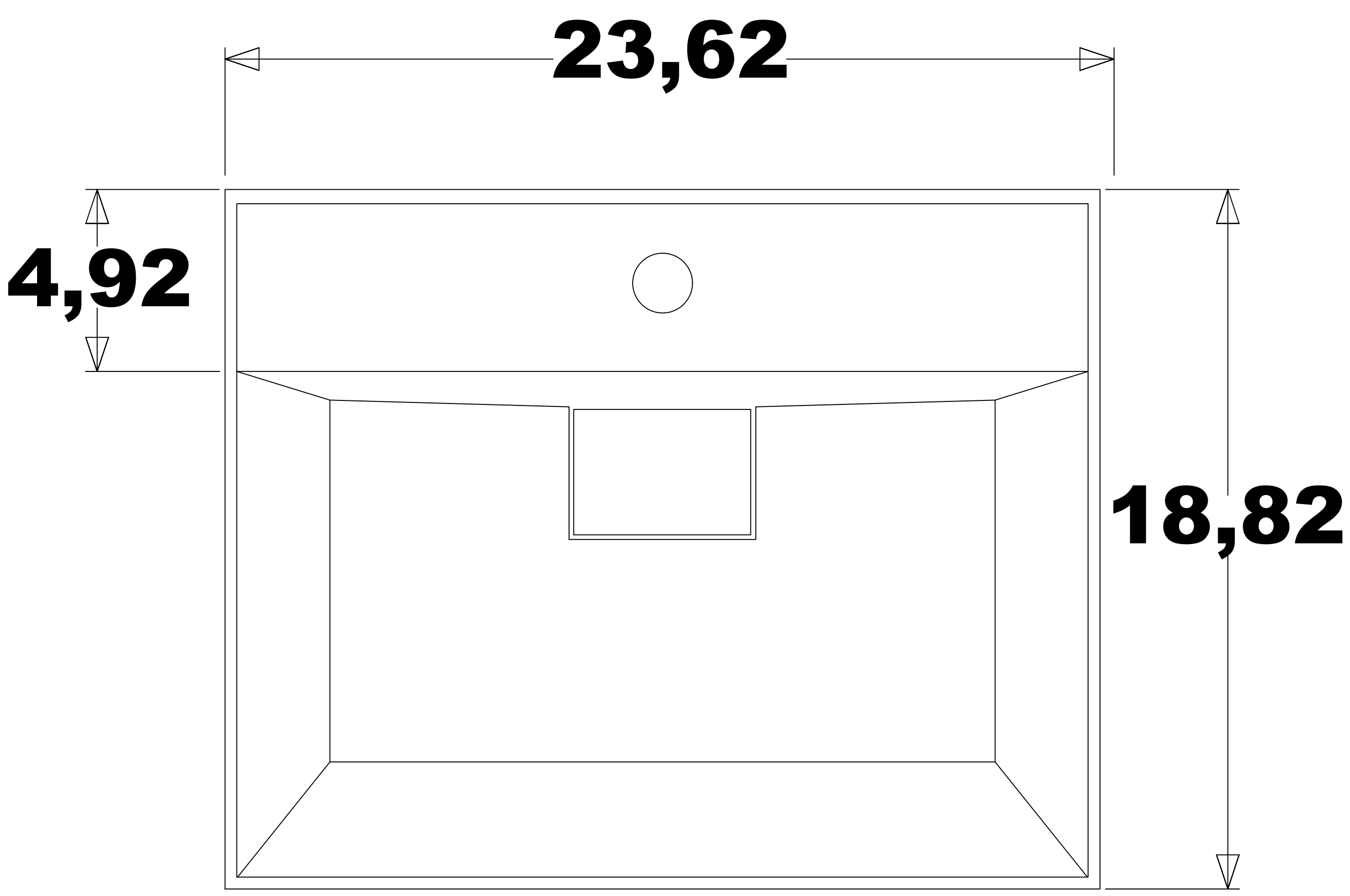
TOP VIEW
