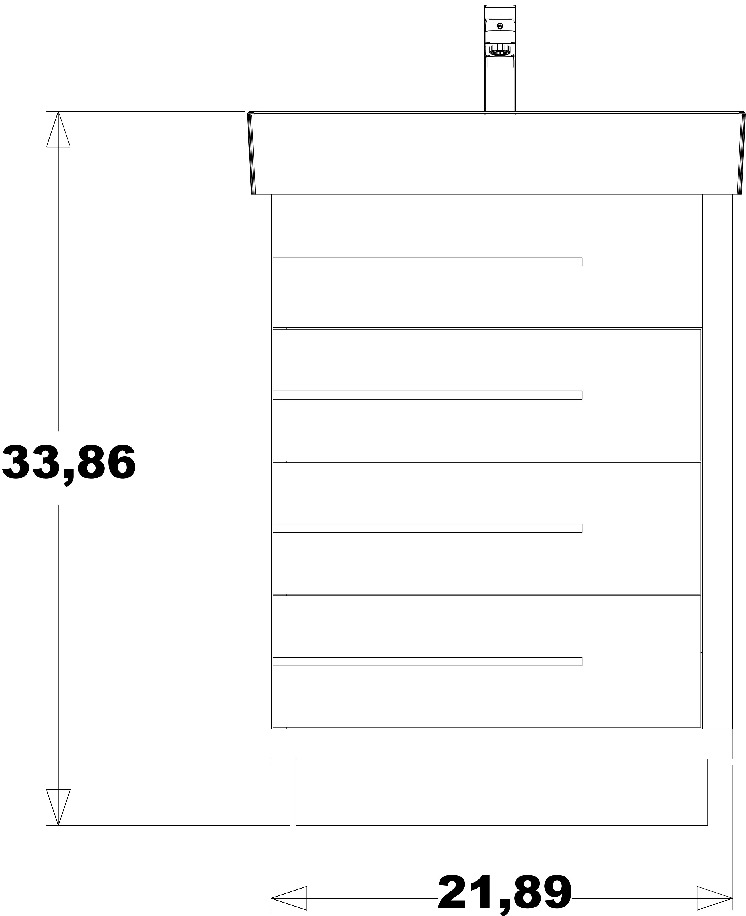
FRONT VIEW
