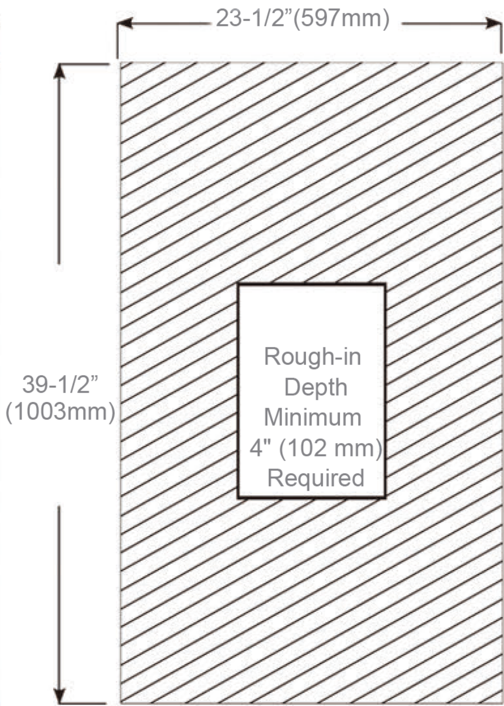
Rough-in Dimensions
