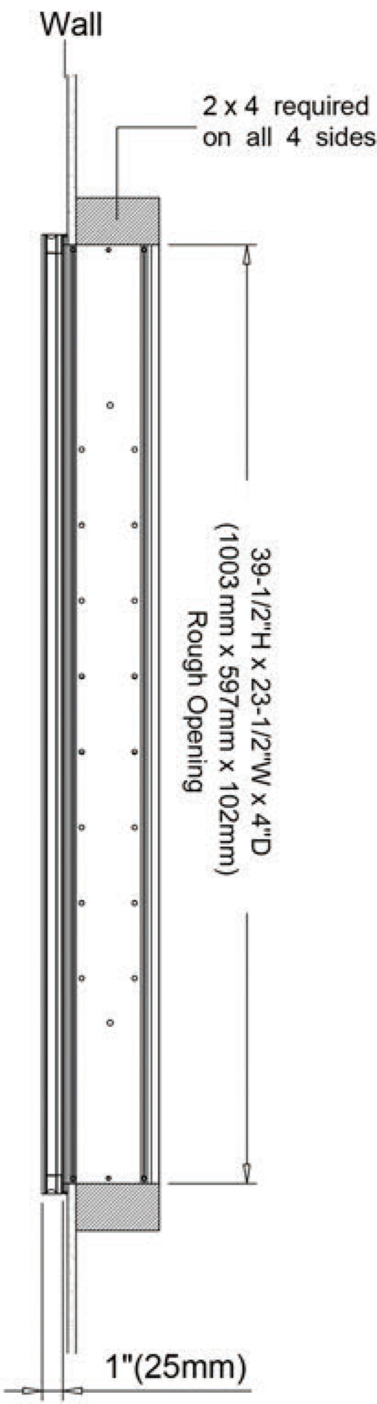
Recessed Mount
