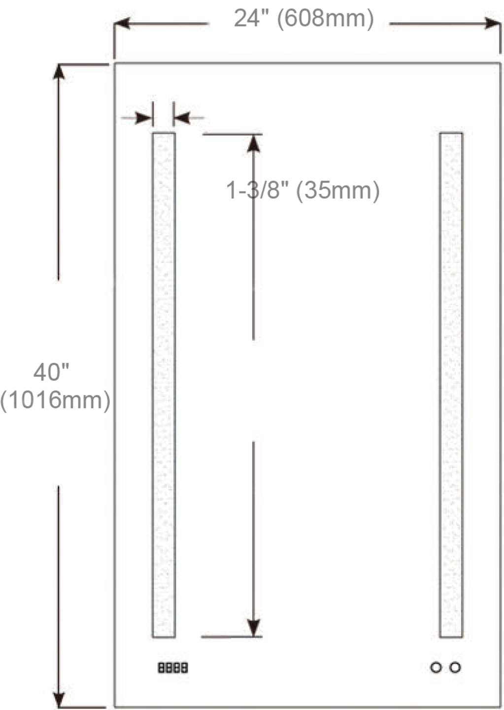
Cabinet Dimensions
