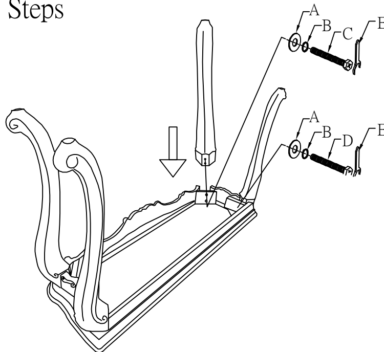
LEG 4PCS
