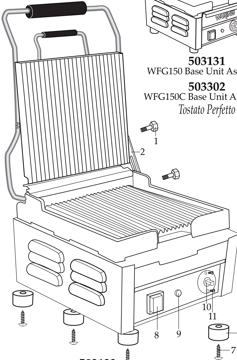
503132 WPG150 Base Unit Assembly
