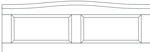
1 Headboard panel (147 x 50.7cm)
