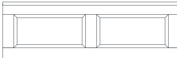
9 Footboard panel (147 x 47.7cm)
