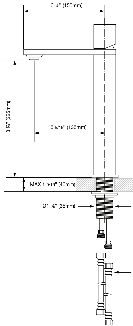
FRONT VIEW
