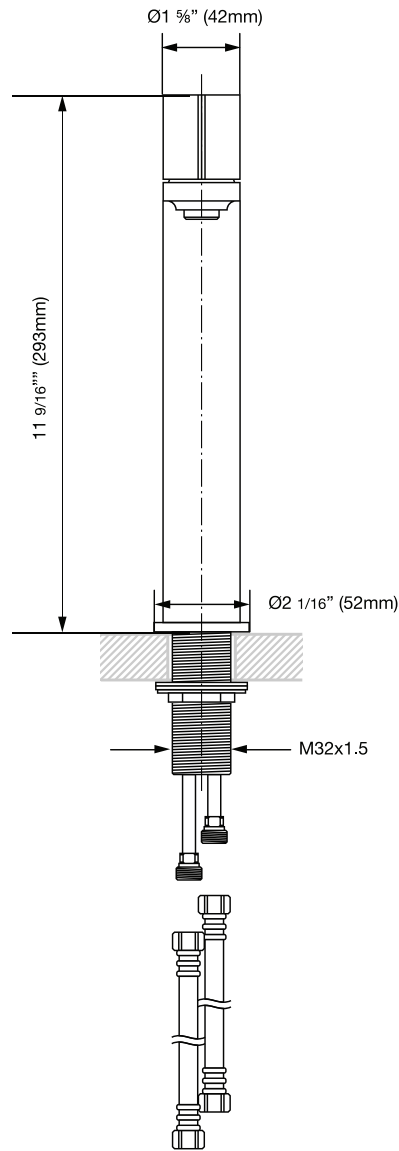
SIDE VIEW
