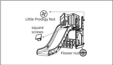
8 Attach the U-shaped side panel⑫ to the 2-lug platform⑤ and the other side of the slide
