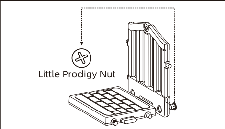
7 Assemble platform baffle⑬ and 2-lug platform⑤
