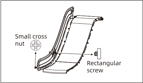
10 Install the slide handrail③ on one side of the slide
