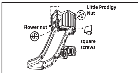
7 Attach the assembled slide to the large side plate⑨ and align it with the 2-lug platform⑤
