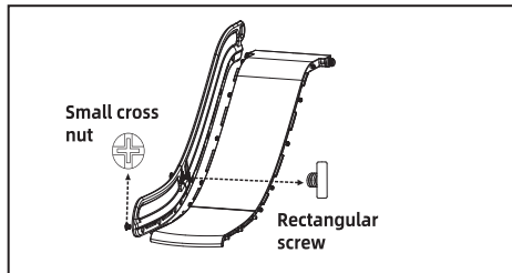
2 Install the slide handrail③ on one side of the slide
