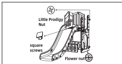
8 Attach the U-shaped side panel⑩ to the 2-lug platform⑤ and the other side of the slide
