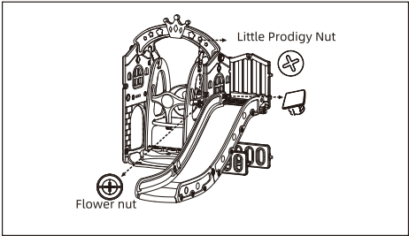
12 Attach the assembled slide to the large side panel⑨
