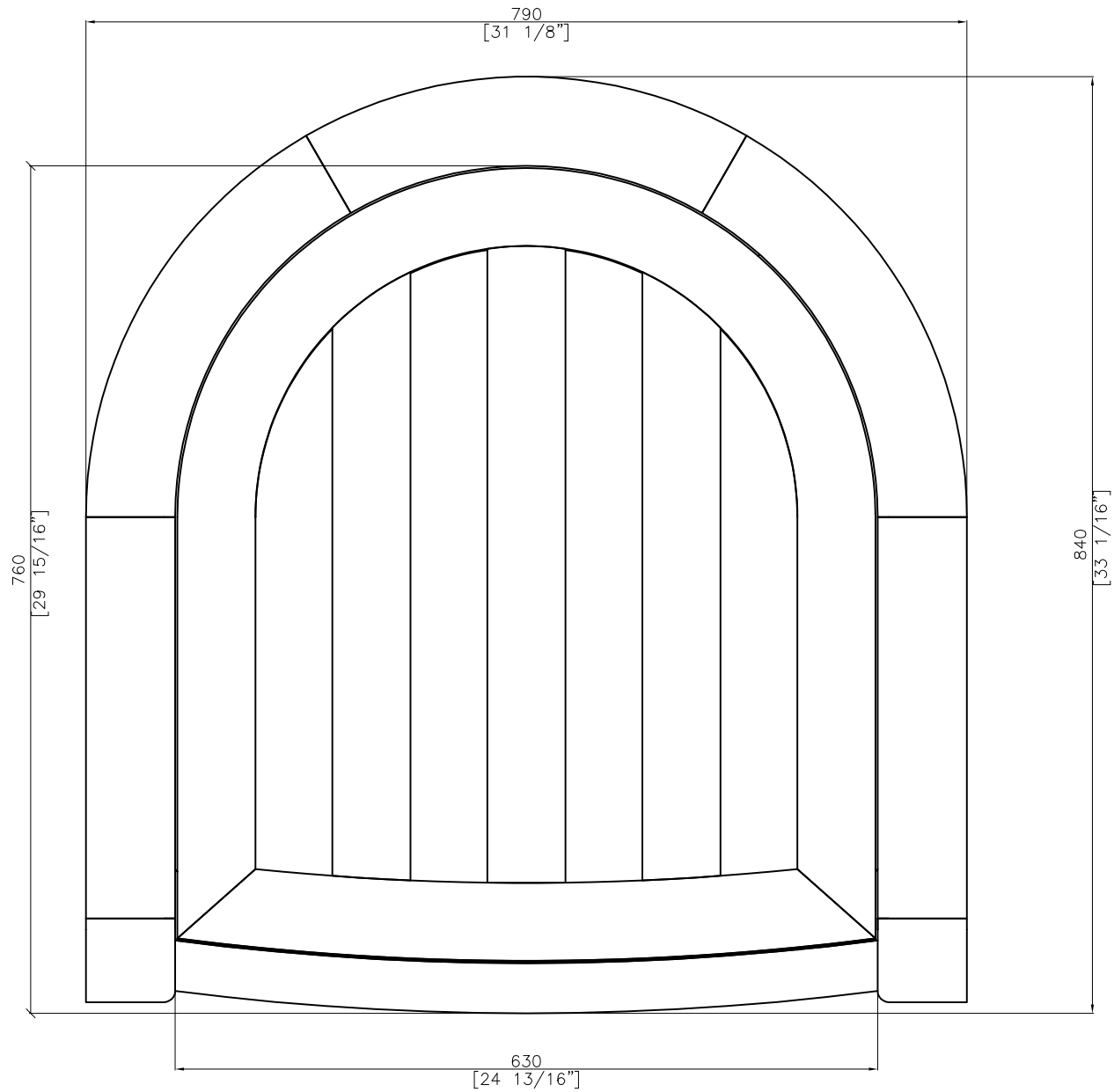
TOP VIEW
