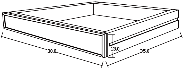
DRAWER DESIGN
