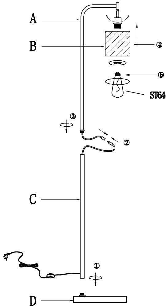
Installation sequence diagram
