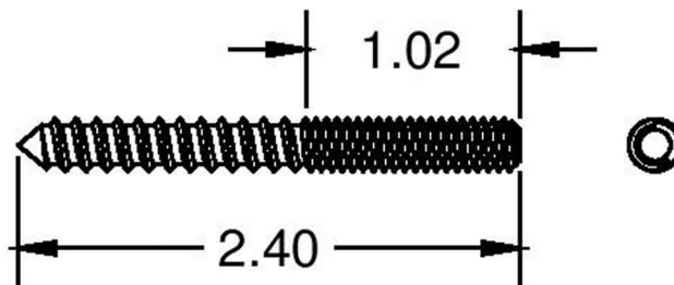
1/4-20 HANGER BOLT
