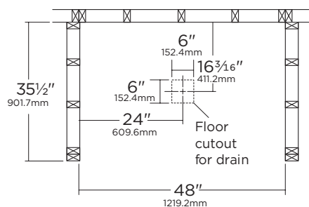
48" x 34" Rectangular Base Fits 48" rough opening
