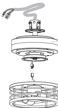
5. Motor Assembly
