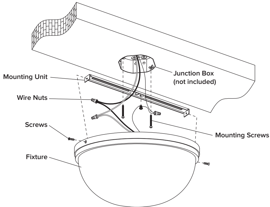
Mounting Screws
