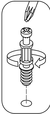
KD Cam
