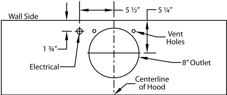
600 CFM B200 Dual Blower (Top View)
