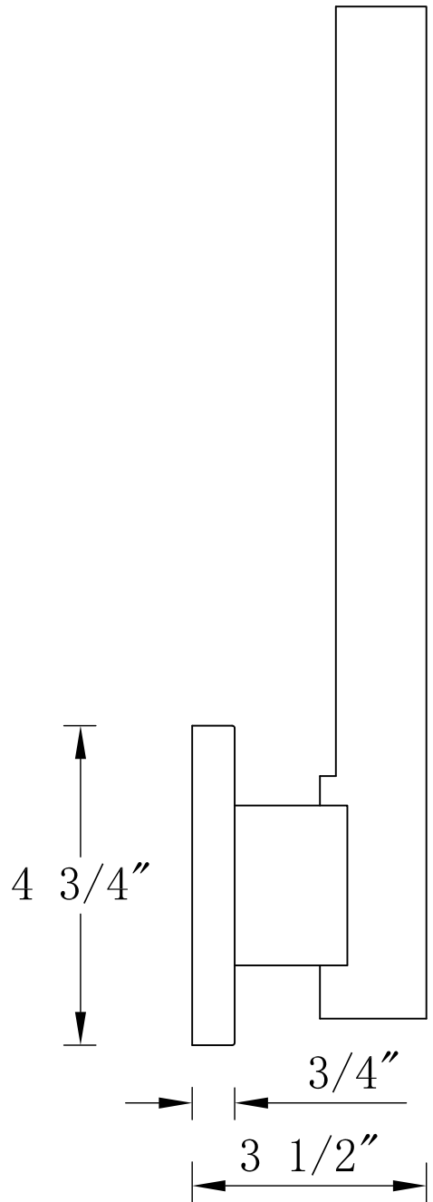
SIDE VIEW
