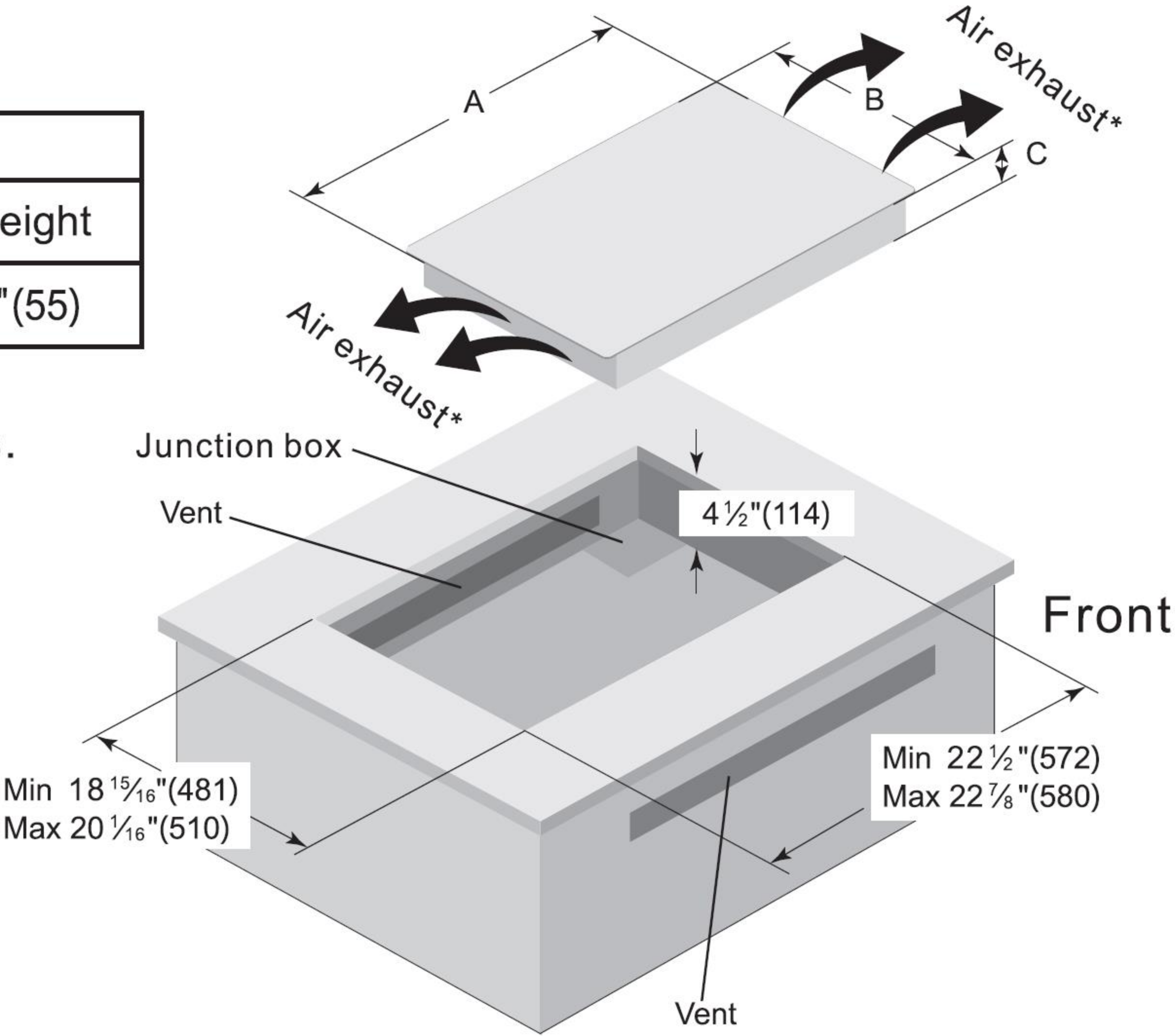
EMPV-IDC24 Cooktop and Cutout Dimension
