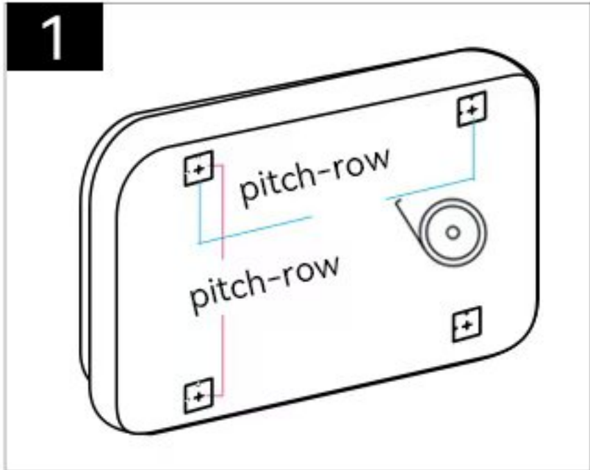
Measure the horizontal and vertical mounting hole spacing of the mirror cabinet.
