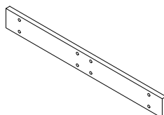
8 (700x75x18mm) X 3
