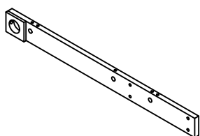
4 (838x75x27mm) X 2
