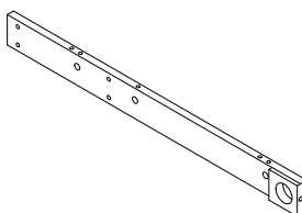
5 (838x75x27mm) X 2
