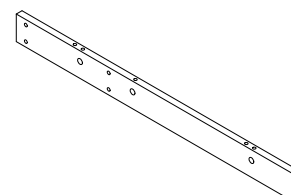
6 (864x75x18mm) X 1
