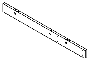
7 (864x75x18mm) X 1
