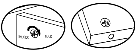
Proper orientation of CAM LOCK
