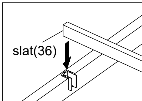
3. Put the slat (36) into the clamp.
