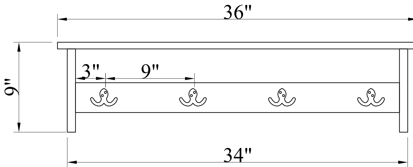
FRONT VIEW
