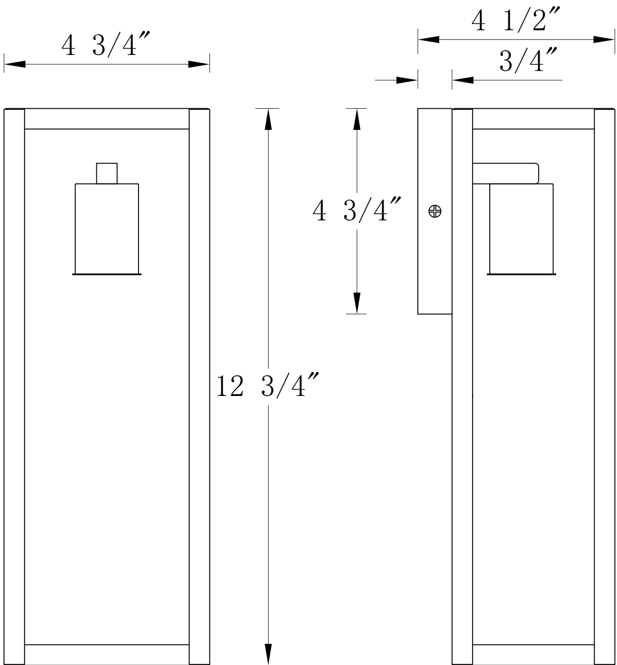
FRONT VIEW
