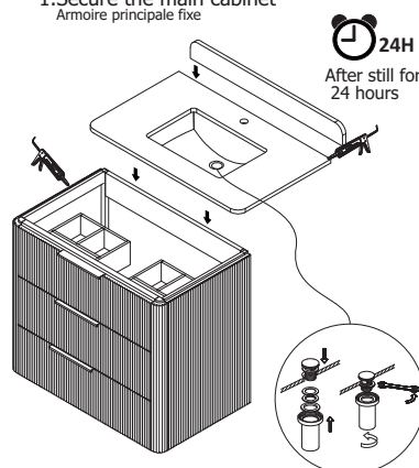
1. Secure the main cabinet Armoire principale fixe
