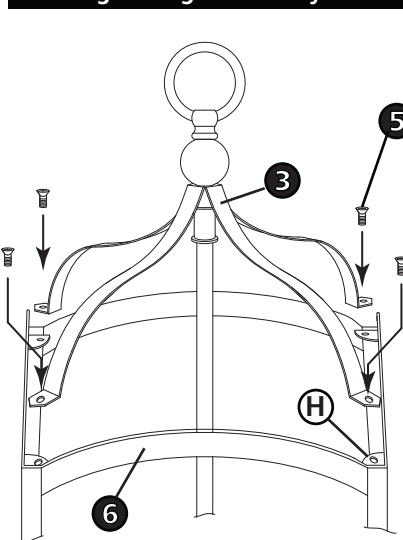
Drawing 1 - Cage Assembly
