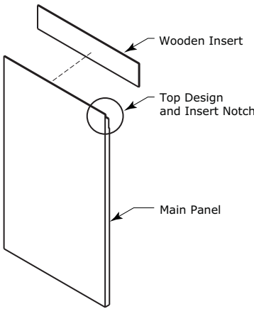
Integrated Panel
