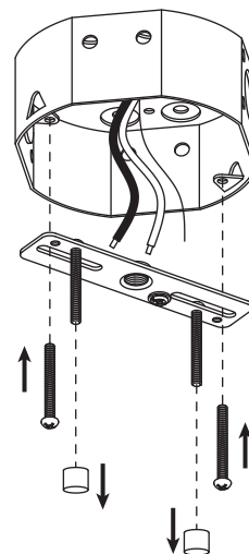
Mounting Screws
