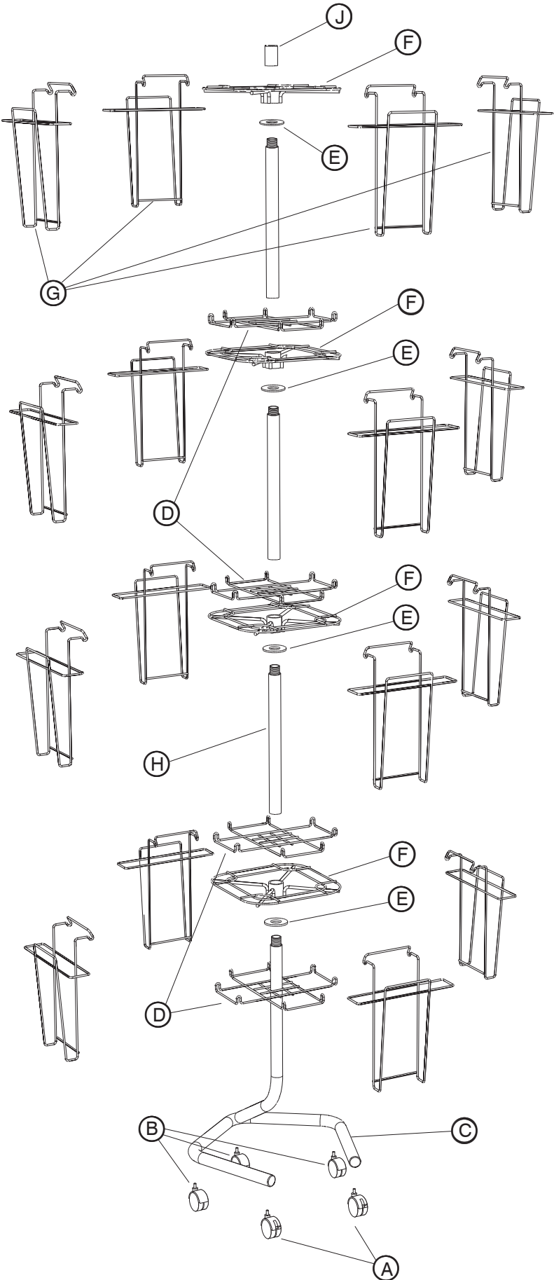
ASSEMBLED UNIT
