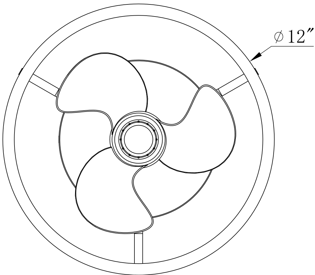
TOP VIEW
